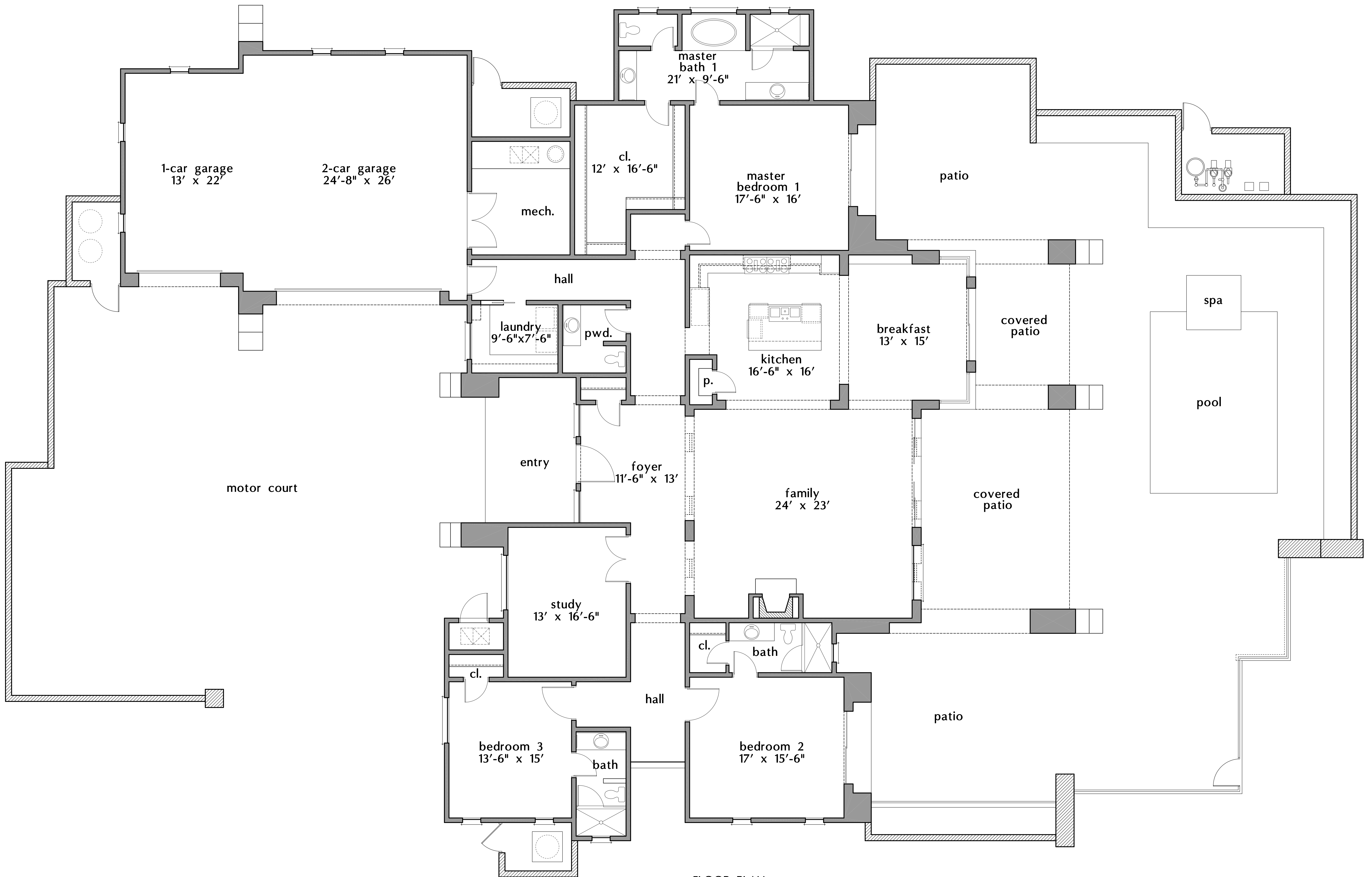
FLOOR PLAN SQ. FT. = 3607 LIVABLE
